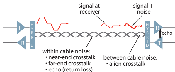
Figure 4: Signal Impairments at the Receiver
